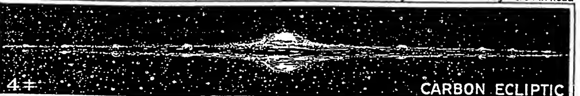
4# . Shown edge on in plane. Note absolute symmetry of ecliptic with no projecting planets. When outer planets project from ecliptic, the element changes to nickel, then copper, zinc, etc. ©
